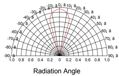
Radiation Characteristics
