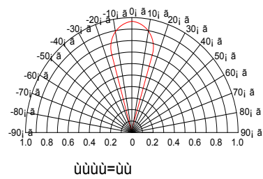
Radiation Characteristics
